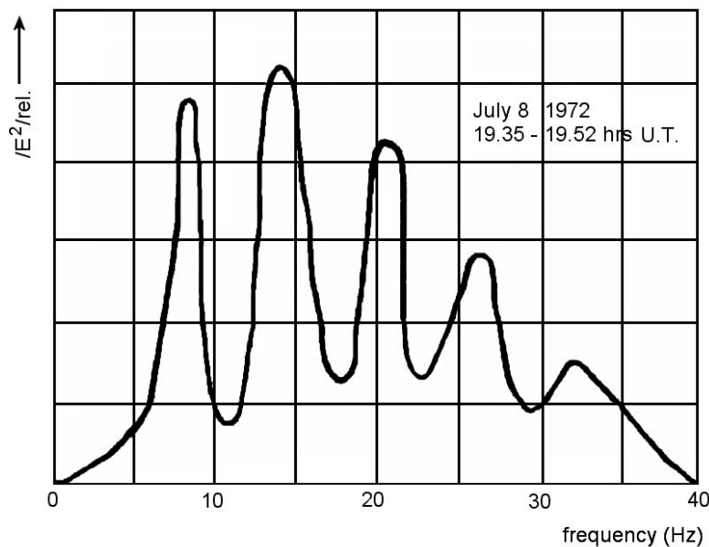
Fig. 3: Spectrum of the vertical electric field of natural signals (noise) in the ELF range
