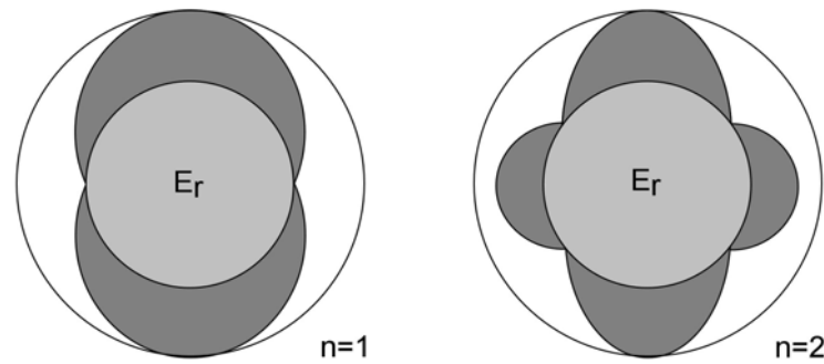
Figure 2: Schumann oscillations
