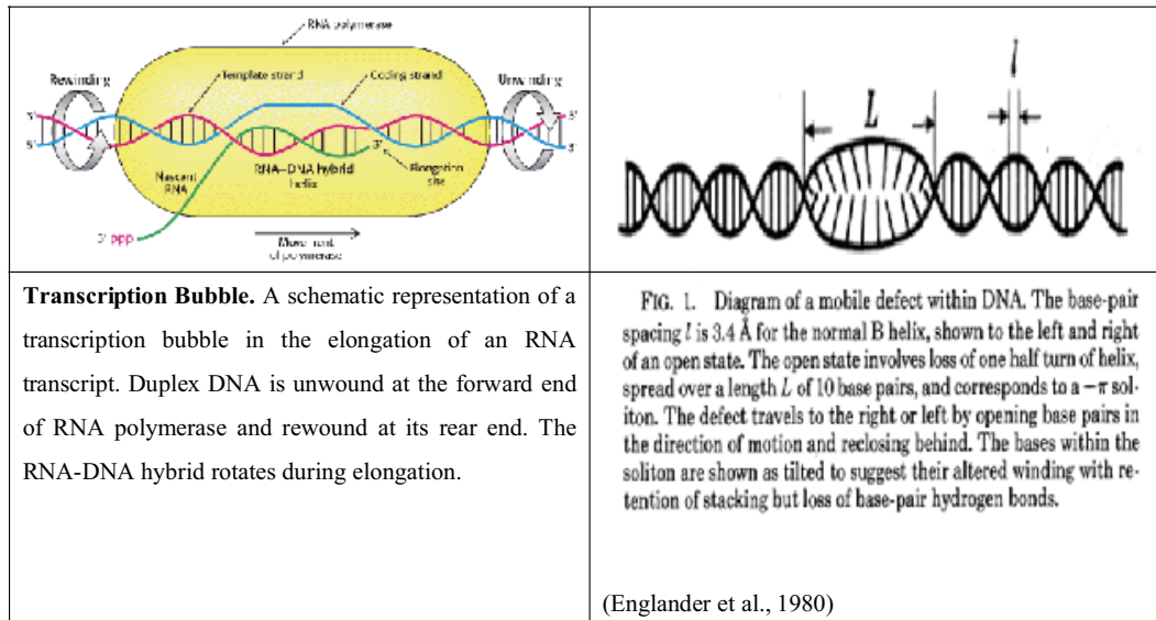
Fig. 6. Solitons in transcription.
